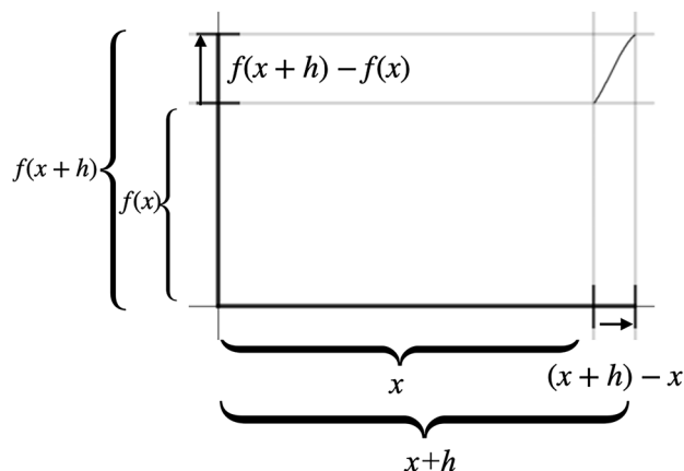
Fig. 1 Variation in the value of x and the corresponding variation in the value of f(x)
